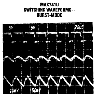
A = MOSFET DRAIN VOLTAGE (5V/div) B = OUTPUT VOLTAGE RIPPLE (AC: 50mV/div) C = INDUCTOR CURRENT (1A/div) CIRCUIT OF FIGURE 7
